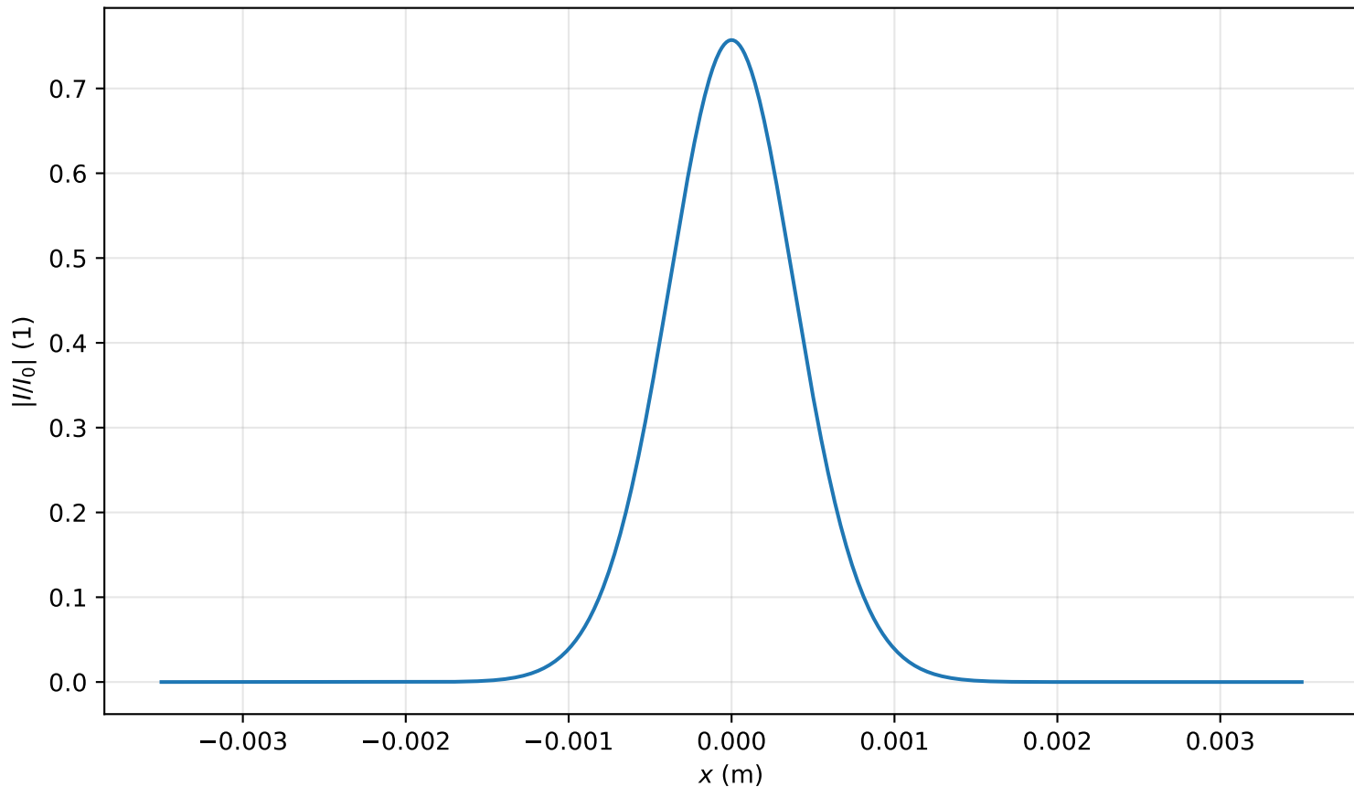
Intensity profile I(x, y = 0, z = 1.433m)/I_0 , P_{in}=0.2P_{cr} , artificial time
